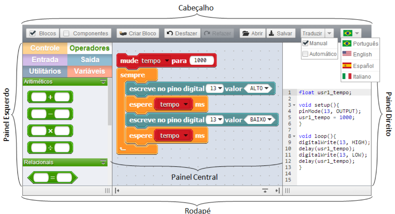
Figura 18: Layout do Ambiente DuinoBlocks
