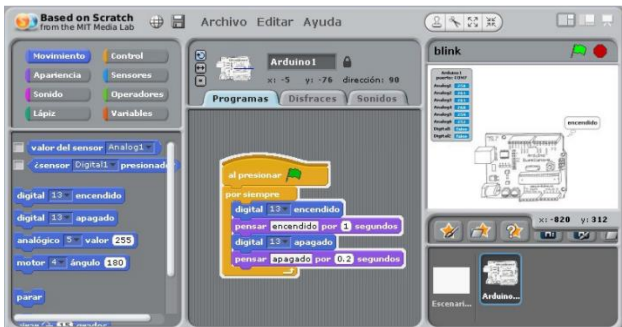
Figura 9: Layout do S4A
