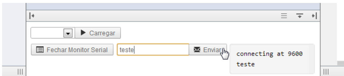
Figura 36: Monitor serial
